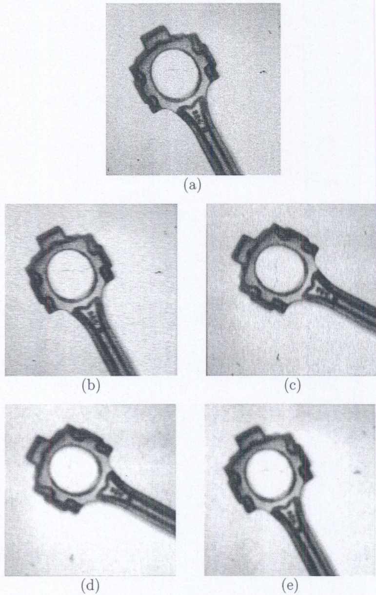
Figure 4.13: The results of separable Gaussian convolution using a single horizontal convolution mask. (a) Original noisy image. (b) Results of convolution with horizontal Gaussian mask. (c) The transposition of (b). (d) The convolution of (c) with the horizontal mask. (e) The transposition of (d). This is the final smoothed image.
