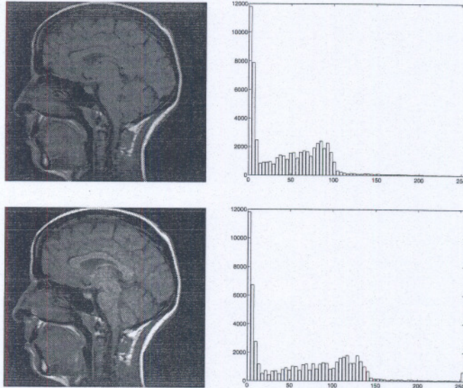
Figure 4.2: The original image has very poor contrast since the gray values are in a very small range. Histogram scaling improves the contrast but leaves gaps in the final histogram. Top : Original image and histogram. Bottom : Image and resulting histogram after histogram scaling.
