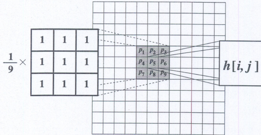
Figure 4.6: An example illustrating the mean filter using a 3 \times 3 neighborhood.
