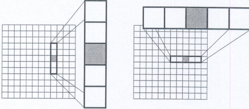
Figure 4.12: An example of the separability of Gaussian convolution. Left : Convolution with the vertical mask. Right : Convolution with the horizontal mask. Note that the origin of each mask is shaded.
