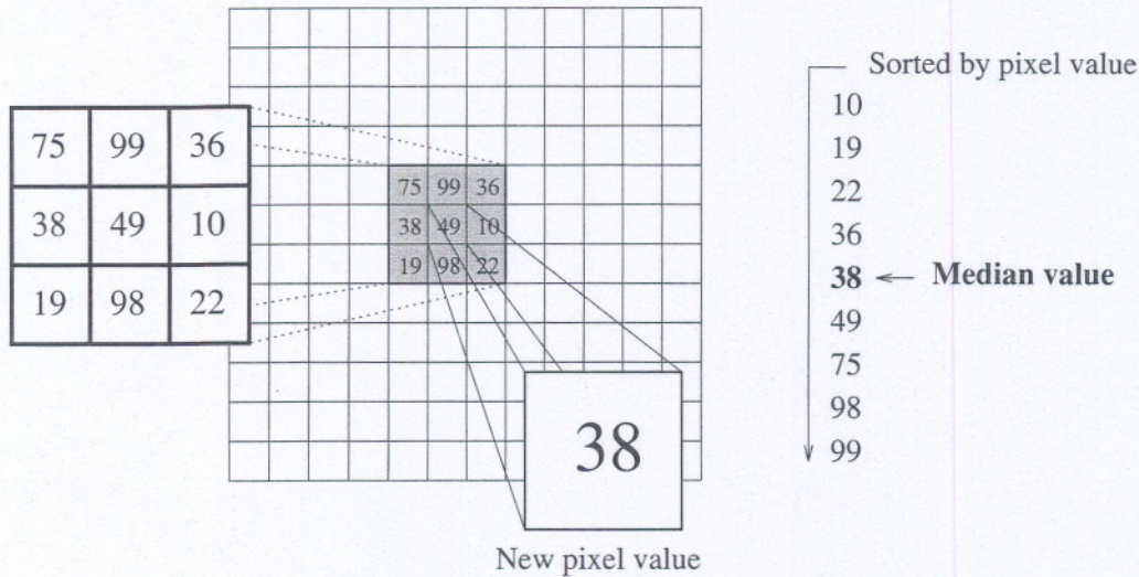
Figure 4.9: An example illustrating the median filter using a 3 \times 3 neighborhood.
