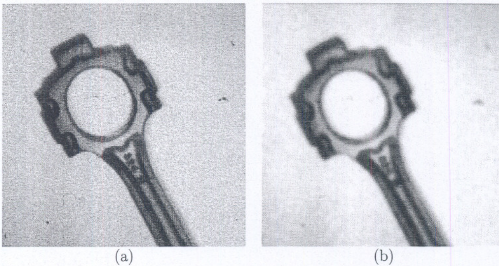
Figure 4.16: The results of smoothing using the 7 \times 7 Gaussian mask. (a) Original image corrupted by Gaussian noise. (b) Smoothed image.
