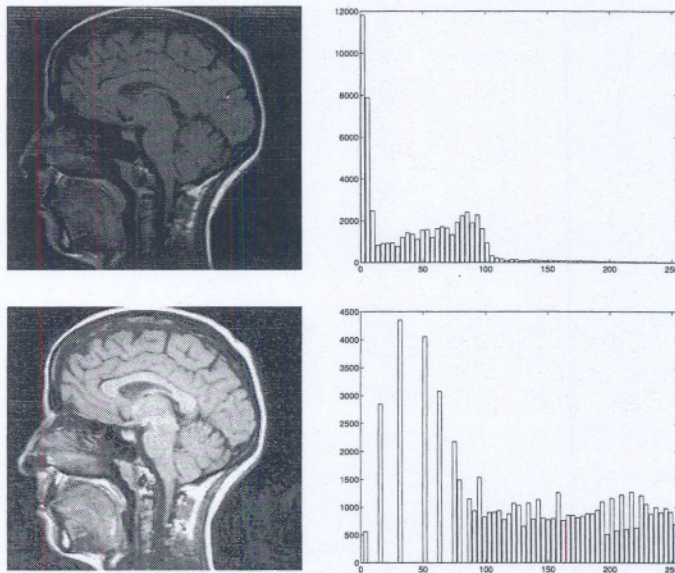
Figure 4.3: The original image has very poor contrast since the gray values are in a very small range. Histogram equalization improves the contrast by mapping the gray values to an approximation to a uniform distribution. However, this method still leaves gaps in the final histogram unless pixels having the same gray levels in the input image are spread across several gray levels in the output image. Top: Original image and histogram. Bottom: Image and resulting histogram after histogram equalization.
