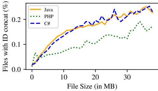
Figure 4: Percentage of unique files with SQL identifier concatenations by file size
