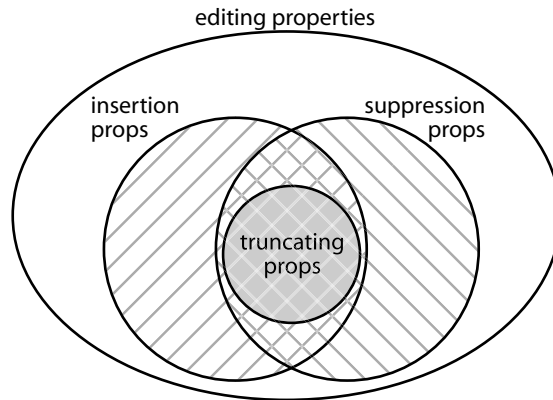
Fig. 3 A taxonomy of effectively enforceable security properties.
