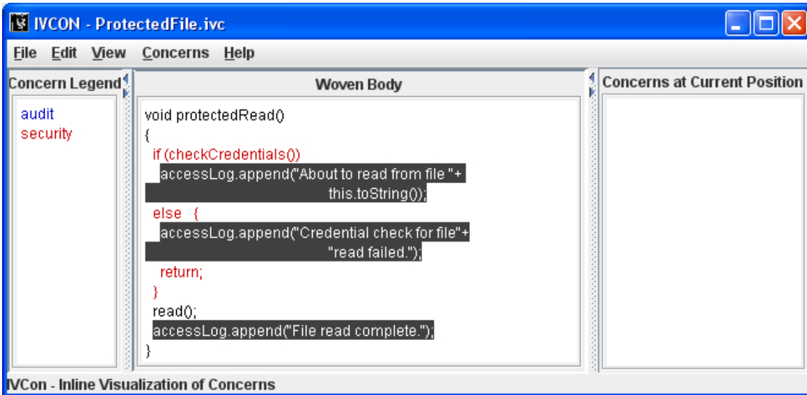
Figure 1. IVCon's woven view of the same code shown in Figure 2
