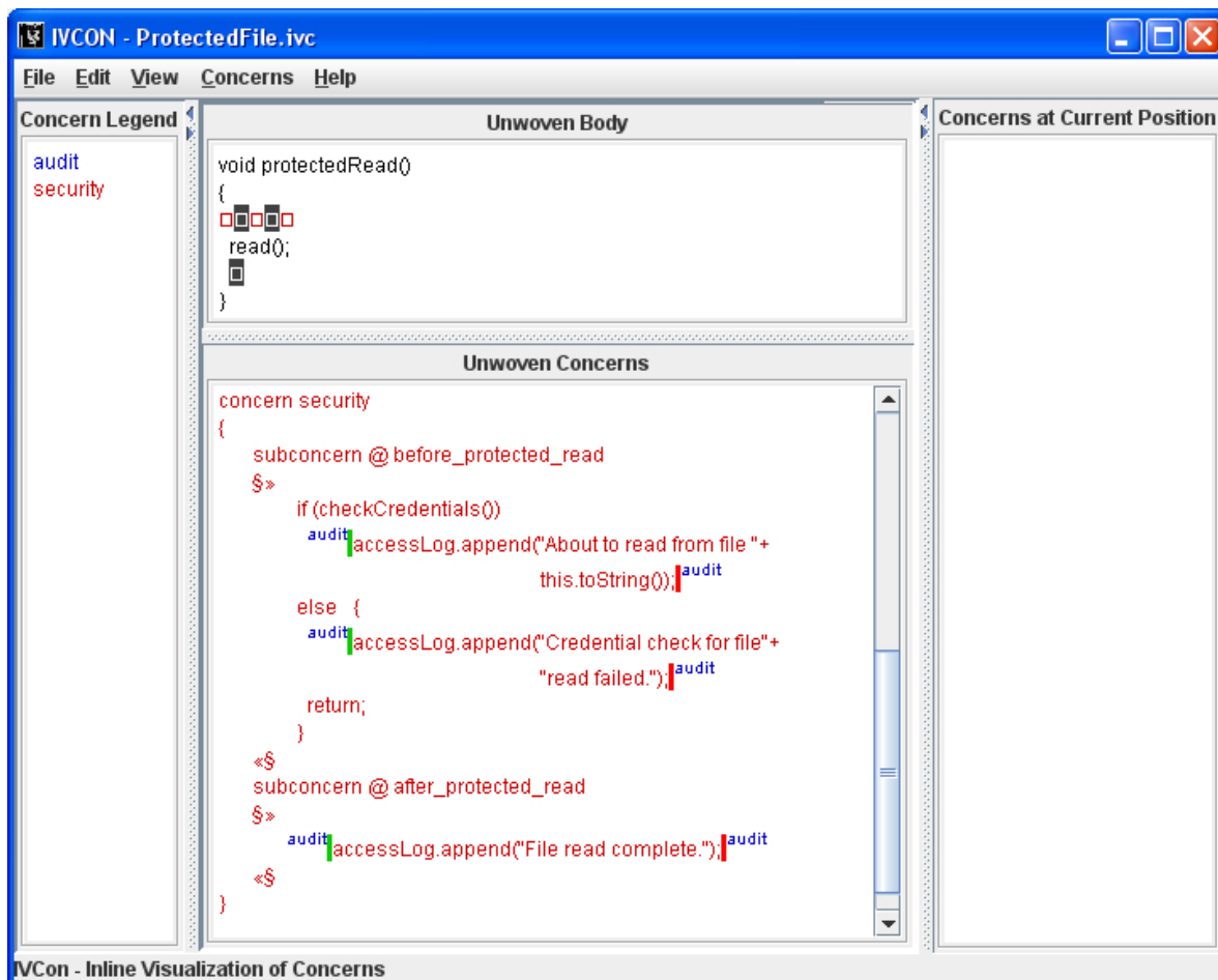
Figure 2. IVCon's unwoven view of the same code shown in Figure 1
