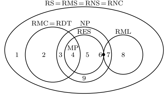
Fig. 5 A hierarchy of reasonable security properties.
