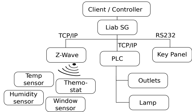
Figure 3. Experiment set-up
