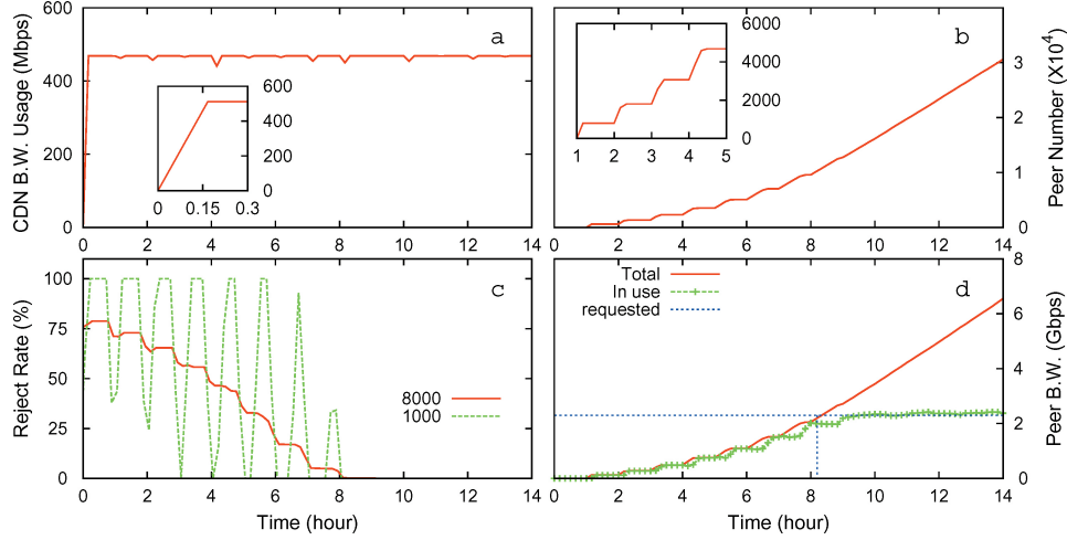
Fig. 5. Performance of a typical hybrid media streaming system. a. Bandwidth usage of CDN servers; b. number of qualified peers; c. system reject rate; d. peer capacity.
