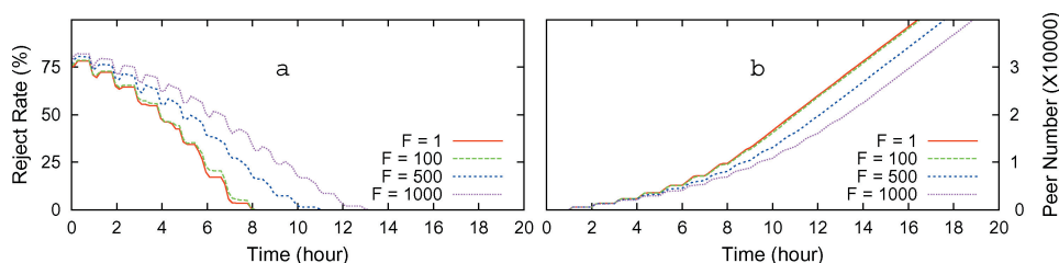
Fig. 7. System performance under different number of media files. a. Smoothed system reject rate; b. number of qualified peers.
